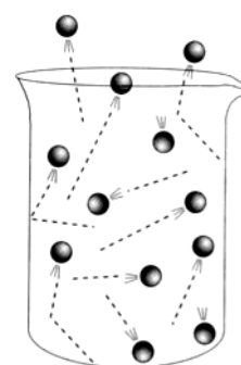
(c) Gases: particles move freely in all directions. Gases are compressible since there is a lot of space between particles.
