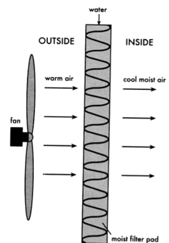
(a) Evaporative air conditioner. Warm air is forced through a moist filter. The evaporating water creates a cooling effect.
