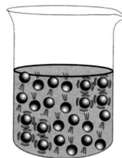
(b) Liquids: particles are free to move within the liquid. Some particles escape the surface to form a vapour.
