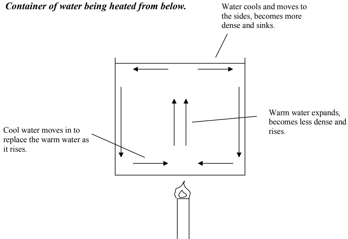
FIGURE 2.3.1 When a liquid or gas is heated, it becomes hotter and less dense so will rise. The colder, denser fluid will fall. As this fluid heats up, it in turn will rise, creating a convection current.
