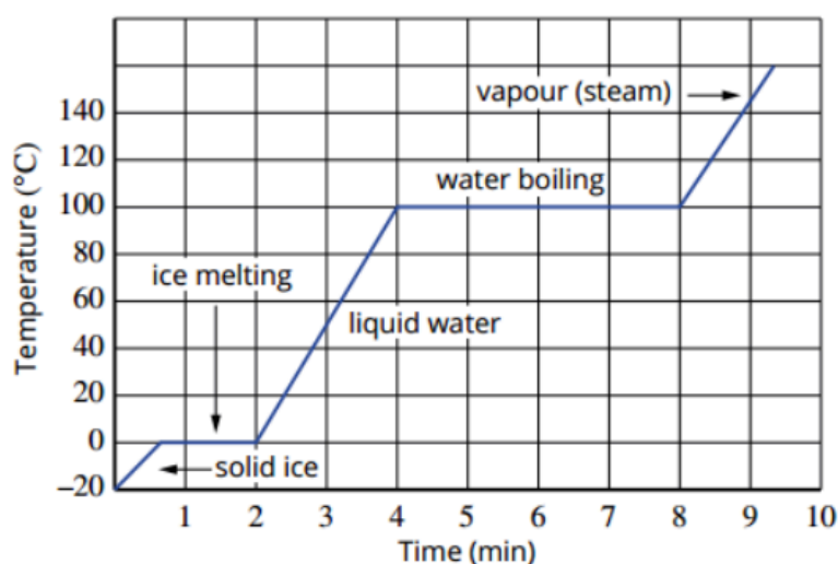
FIGURE 1.3.1 A heating curve for water.
