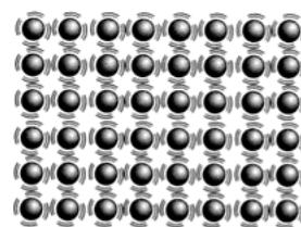
(a) Solids: particles vibrate about fixed positions. Solids have a definite shape.
